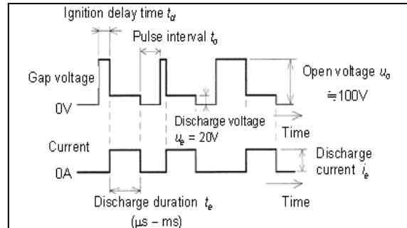
Fig 2: Voltage and Pulse Waveforms of an EDM Machine [3] workpiece takes place and the tool the tool shape is replicated on it.
