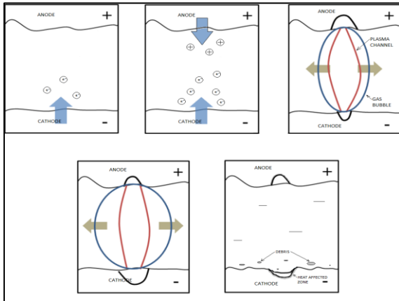
Fig 4: Diagrammatic Representation of EDM Metal Erosion Mechanism
