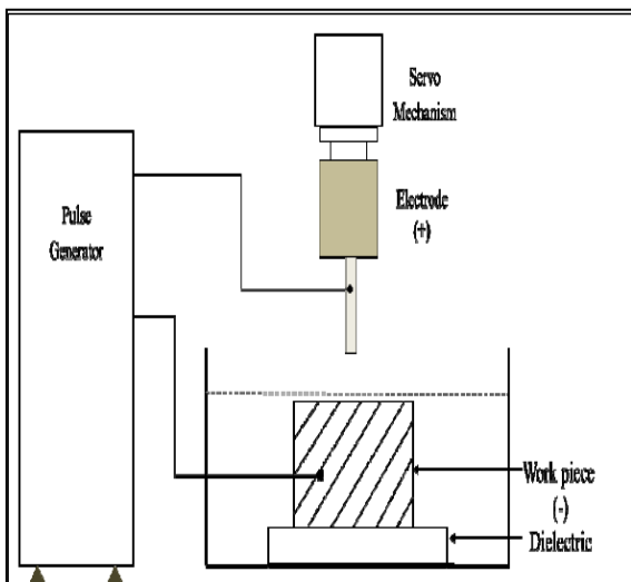
Fig 1: Schematic Diagram of an EDM Machine [2]
