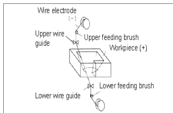
Fig 3: Schematic Diagram of Wire EDM [6]
